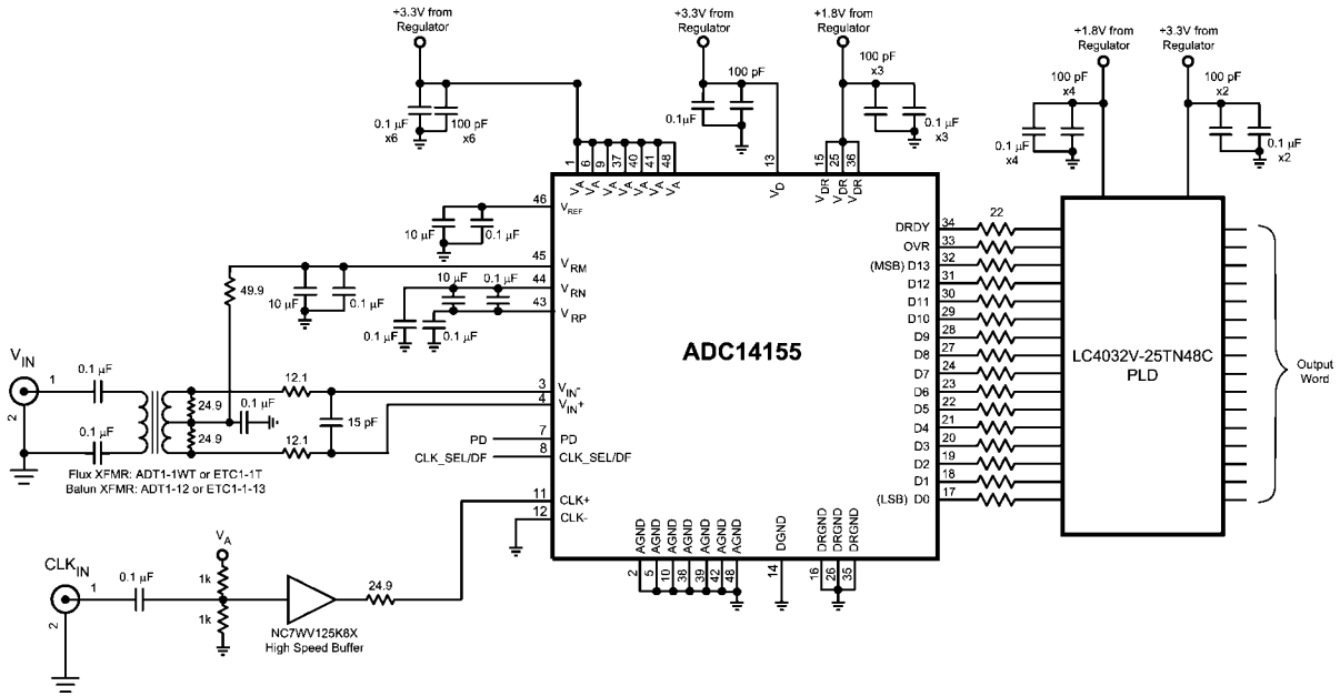
FIGURE 4. Application Circuit using Transformer Drive Circuit
